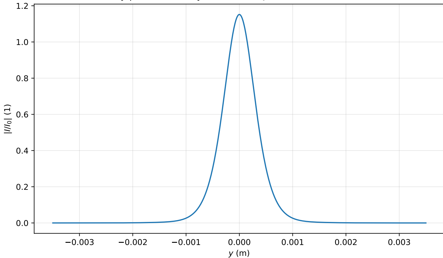
Intensity profile I(x=0, y, z=2.786)/I_0 , P_{in}=0.8P_{cr} , artificial time
